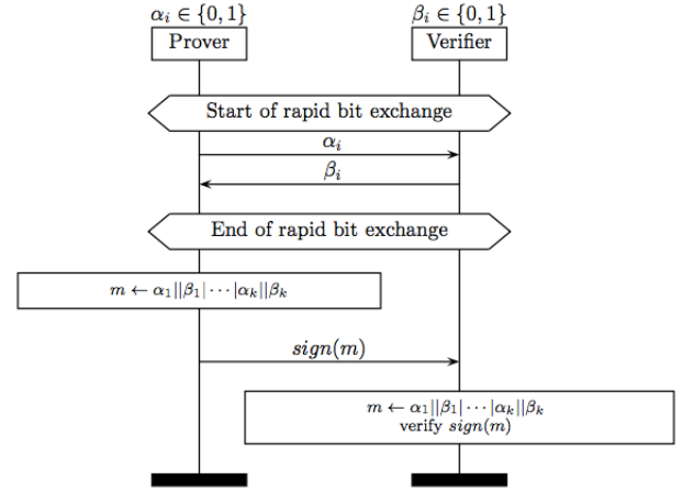
Fig. 2. Brands and Chaum Distance Bounding Protocol [14]
